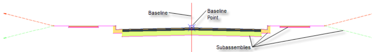
Figure 2. An assembly is made of up a combination of subassemblies such as sidewalks, curb, and lanes.
