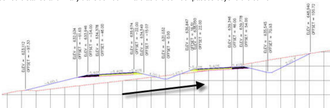
Figure 18. In the example above, the LaneOutsideSuper subassembly is using data from the Outside Lane column, in the Alignment properties.
