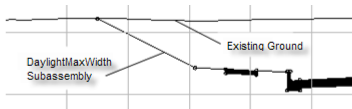
Figure 12. Daylight subassemblies use a surface target parameter to seek out and intersect surfaces based on input parameters. For example, DaylightMaxWidth Subassembly analyzes whether a cut or fill situation exists, and then uses input parameters to tie into a surface.
